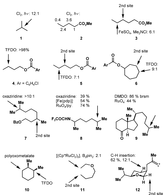
Scheme 1. Electron-withdrawing groups influence the site of C–H activation. B_2pin_2 = bis(pinacolato)diboron, Bz = benzoyl, Cp^* = C_5Me_5 , DMDO = dimethyldioxirane, pdp = 1,1'-bis(2-pyridinylmethyl)-2,2'-bipyridine, py = pyridine, TFDO = methyl(trifluoromethyl)dioxirane; brsm = based on recovered starting material.
