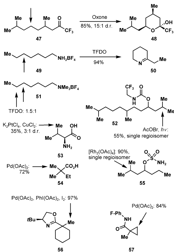
Scheme 8. A number of directing groups may be employed in C–H activation.
