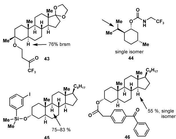
Scheme 7. Directed oxidations offer an opportunity to effect positional selectivity.
