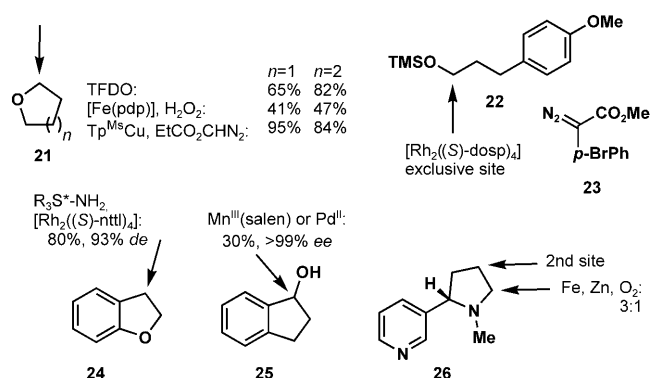
Scheme 3. Hyperconjugation by heteroatoms activates neighboring C-H bonds. dosp = N -( p -dodecylphenylsulfonyl)proline, Ms = mesyl, nttl = N -1,8-naphthoyl- tert -leucine, Tp Ms = hydrotris(3-mesityl)pyrazolyl-borate.
