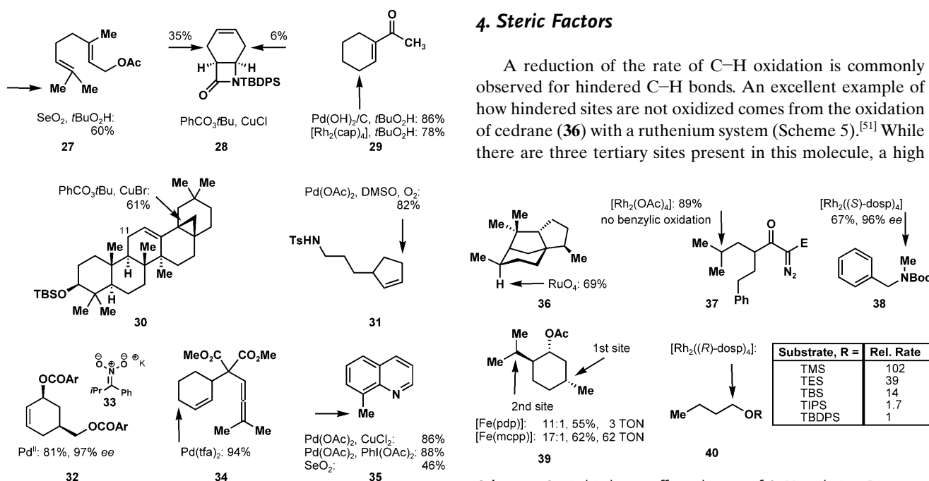
Scheme 4. Oxidation of allylic and benzylic systems. Ts = 4-toluenesulfonyl, TBS = tert -butyldimethylsilyl, cap = caprolactamate, tfa = trifluoroacetic acid.
