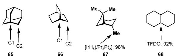
Scheme 10. Unique geometries of bicyclic systems results in varied selectivity.
