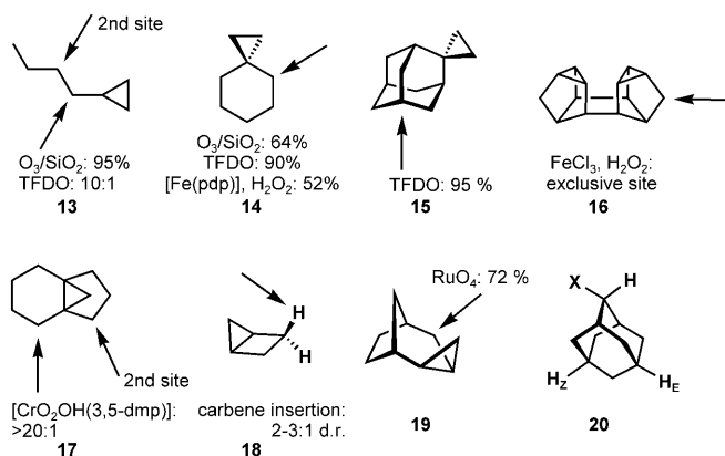
Scheme 2. Hyperconjugation by cyclopropanes activates neighboring C-H bonds. dmp = dimethylpyrazole.
