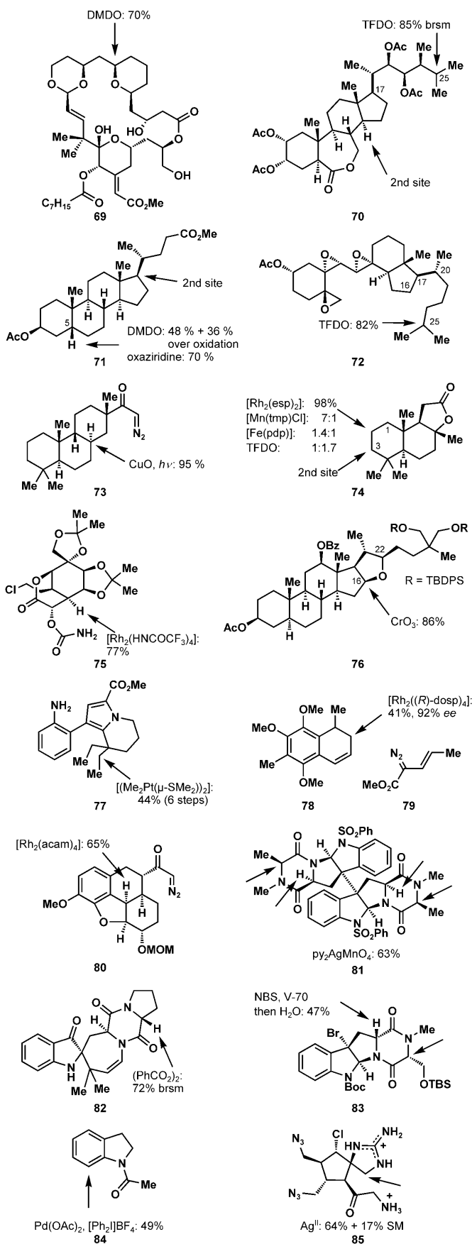
Scheme 11. Additional examples of C–H oxidation. acam = acetamide, esp = \alpha,\alpha,\alpha,\alpha -tetramethyl-1,3-benzenedipropionic acid, MOM = methoxymethyl, NBS = N -bromosuccinimide, tmp = 5,10,15,20-tetramethylporphyrinato; SM = starting material.
