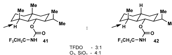
Scheme 6. Strain release may be an important factor in controlling site selectivity in C–H activation reactions.
