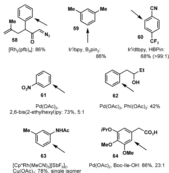
Scheme 9. C–H activation of sp^2 centers presents unique challenges. bpy = 2,2'-bipyridine, dtbpy = 4,4'-di- tert -butyl-2,2'-bipyridine, pfb = perfluorobutyrate.
